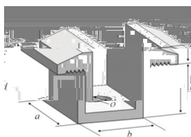
Figure 1 Schematic Diagram of Intermediate Clamp
